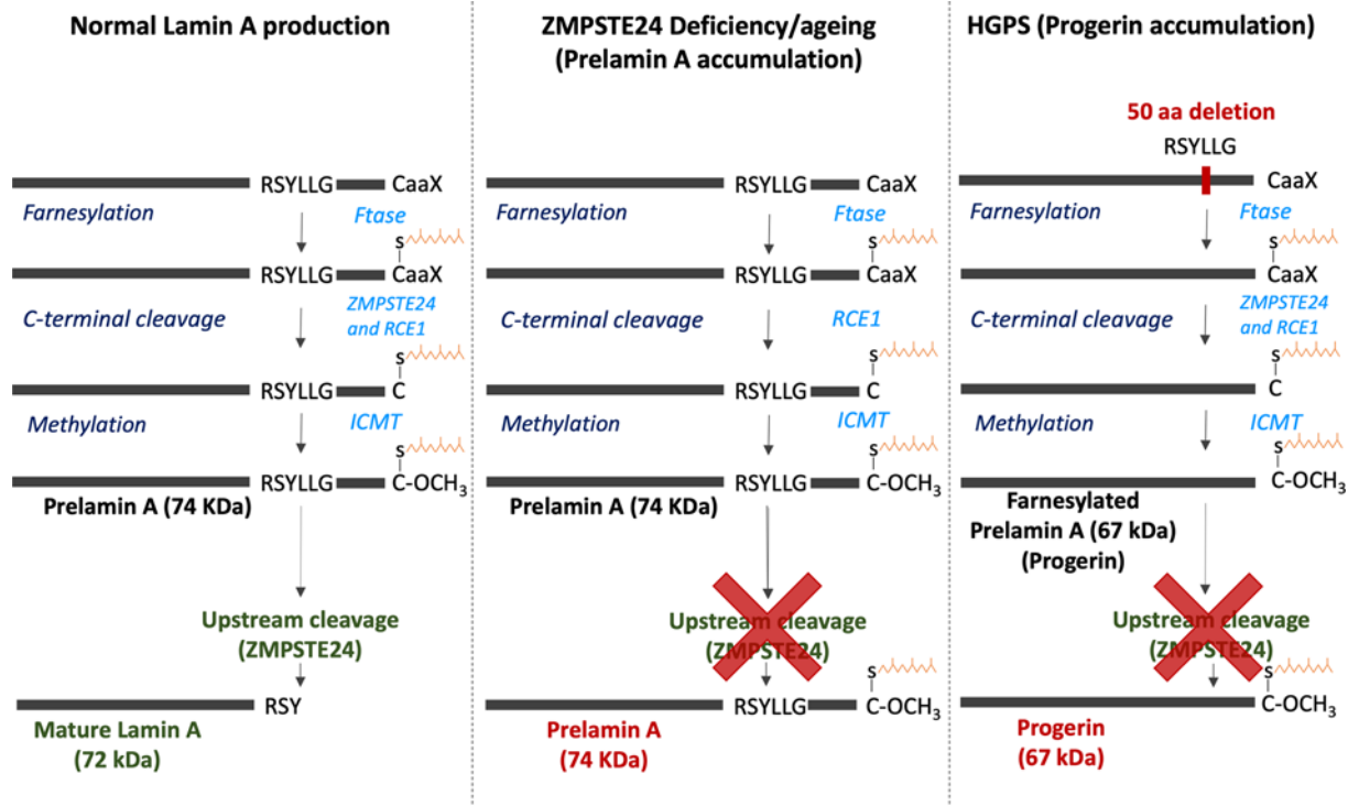
Figure 2. Production of Lamin A, Progerin and Prelamin A from the LMNA gene
