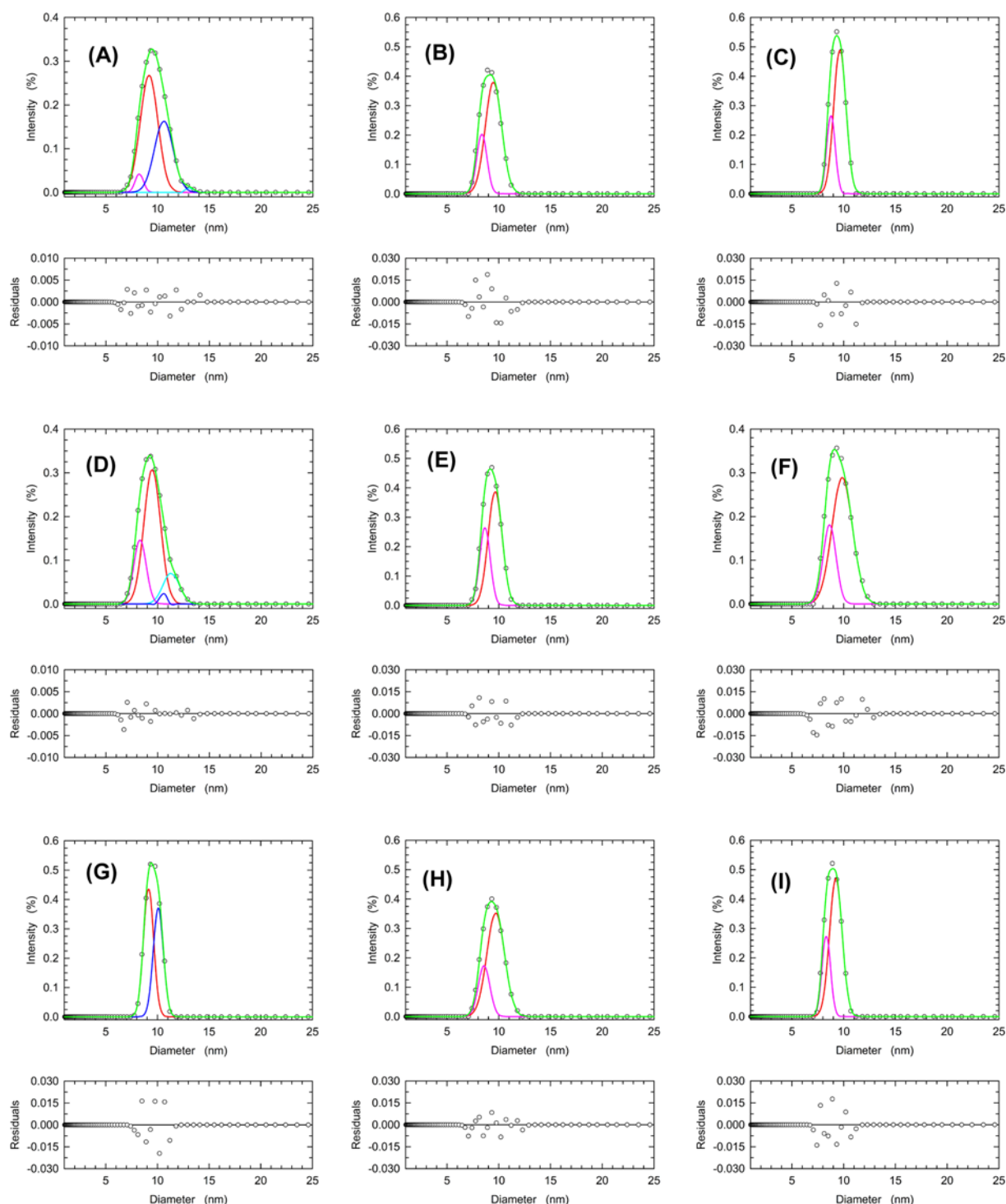
Figure 7. Relative abundance of recombinant human LDH-A tetramer, dimer, and monomer as a function of pH and enzyme concentration
