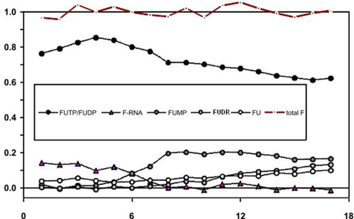
Figure 6. Time evolution of the relative concentration of particular fluorinated species
