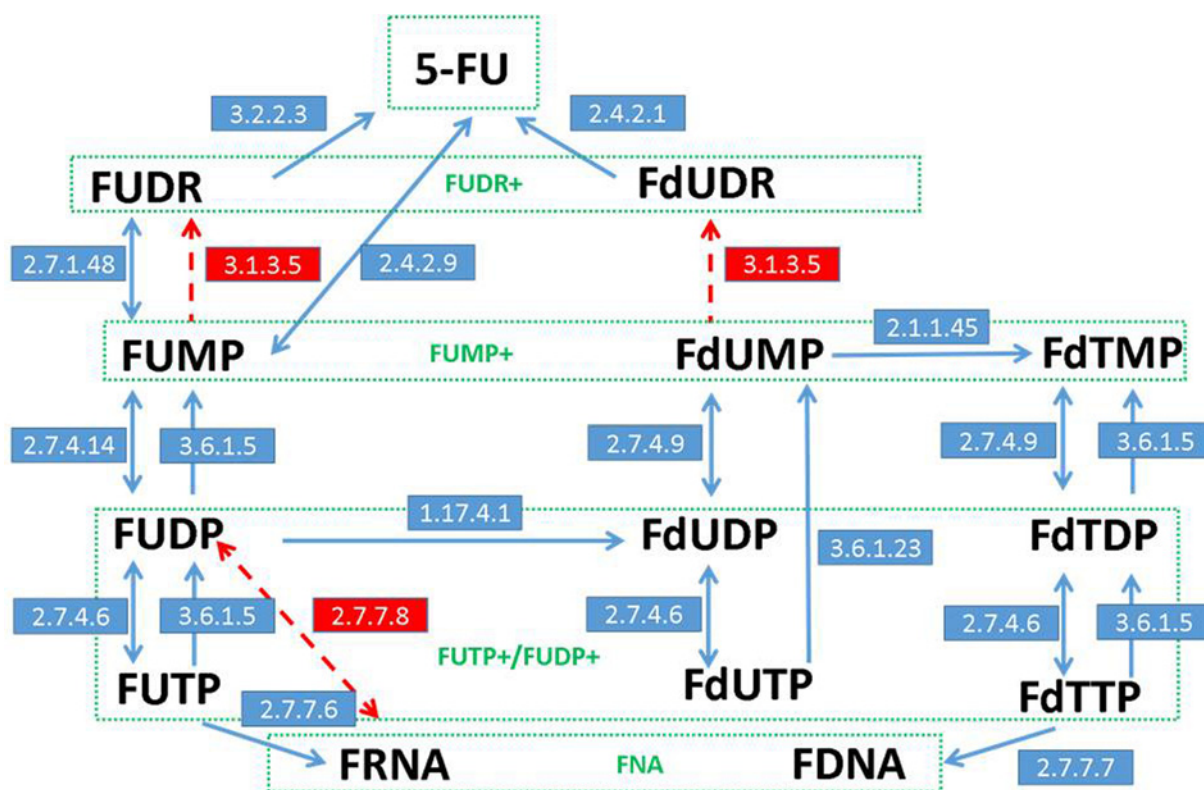
Figure 2. The general schema of the proposed kinetics model of 5-FU metabolism
