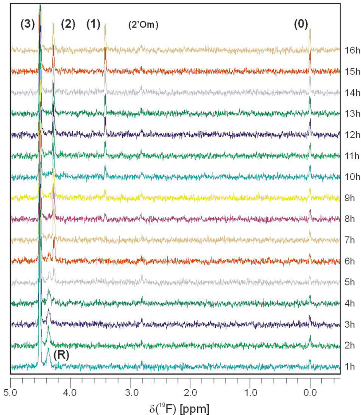
Figure 5. Time evolution of ^{19}\text{F} NMR spectrum
