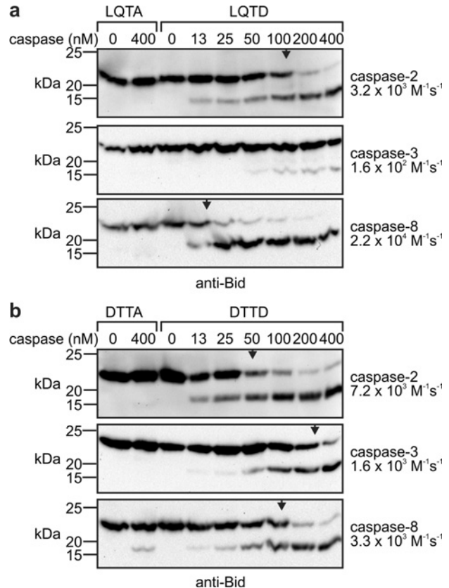
Figure 3 A Bid variant bearing the DTTD cleavage site is efficiently cleaved by caspase-2
