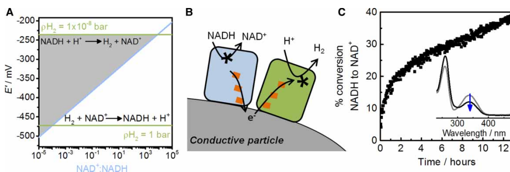
Figure 8. Oxidation of \text{NADH} to \text{NAD}^+ coupled to \text{H}_2 generation on carbon particles.
