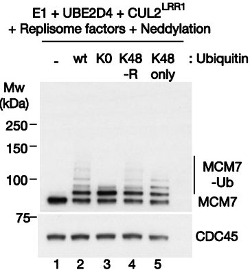
Polyubiquitylation of CMG-MCM7 by UBE2D4 is inefficient and is independent of lysine 48 of ubiquitin. Reactions containing UBE2D4 were performed as in Figure 2A, but in the presence or absence of the indicated variants of ubiquitin.
