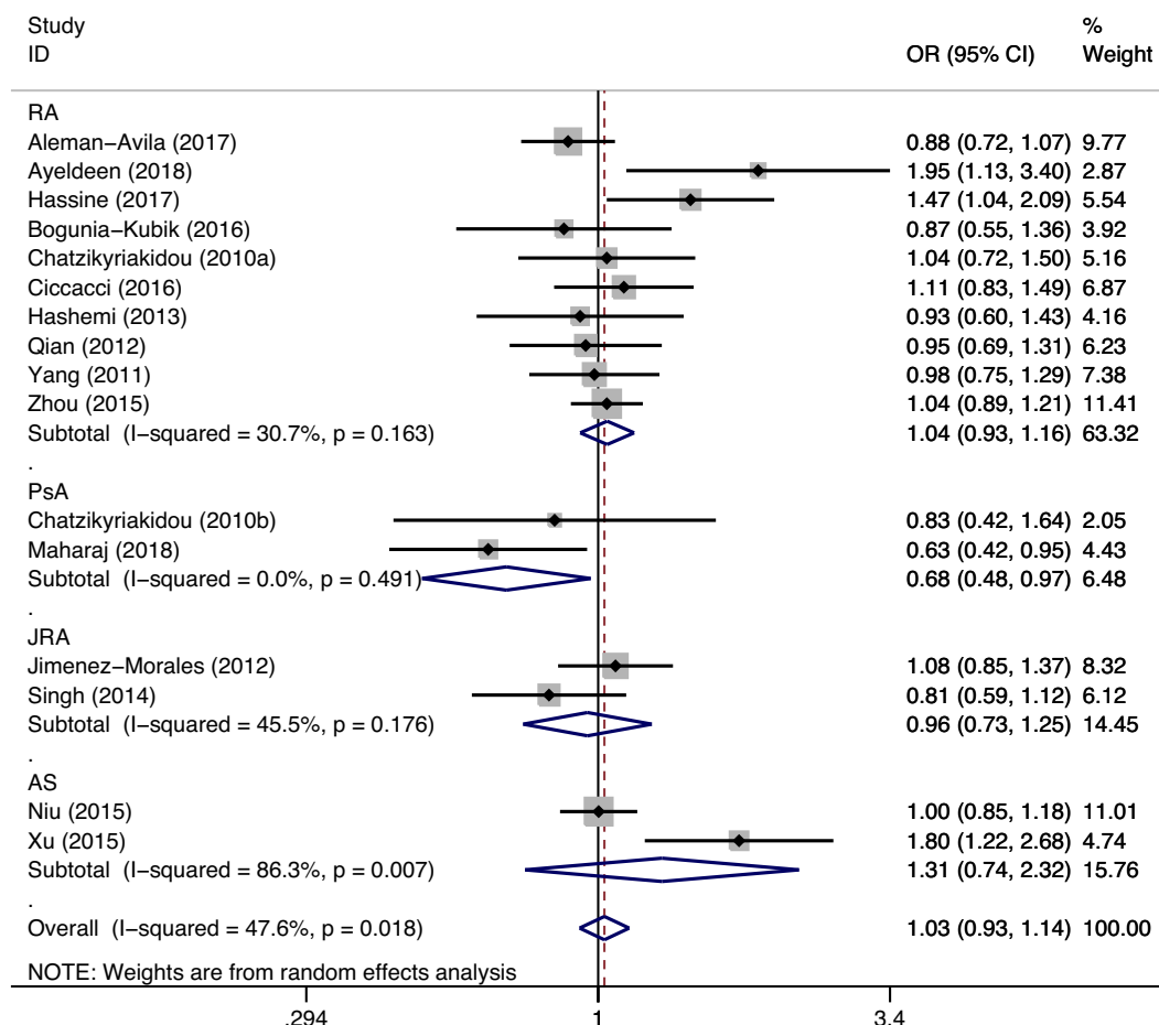
Figure 2. Forest plot of arthritis risk associated with miR-146a rs2910164(G/C)polymorphism in allelic model (G versus C) for the analysis by diseases
