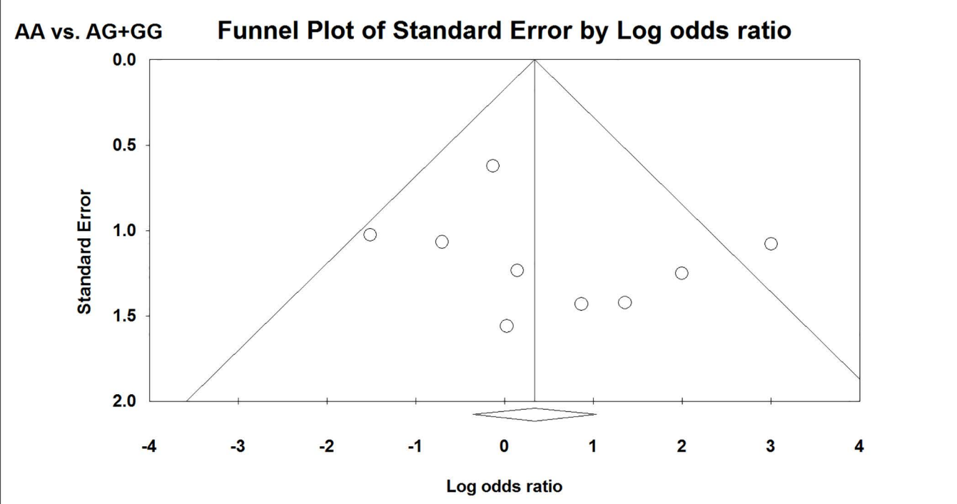
Figure S13: Assessment of publication bias shown with Funnel plots in studies assaying odds of INH induced hepatotoxicity with the NAT2 857G>A (rs1799931) gene polymorphism for overall analysis (Odds ratio against standard error in different genetic models).
