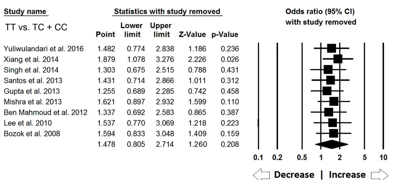
Figure SI4: Sensitivity analysis of NAT2 481C>T gene polymorphism with overall INH induced hepatotoxicity risk to evaluate the influence of each individual study on the pooled OR by deleting one single study each time for the overall analysis (for all the genetic models). Black square represents the value of OR and the size of the square indicates the inverse proportion relative to its variance. Horizontal line is the 95% CI of OR.
