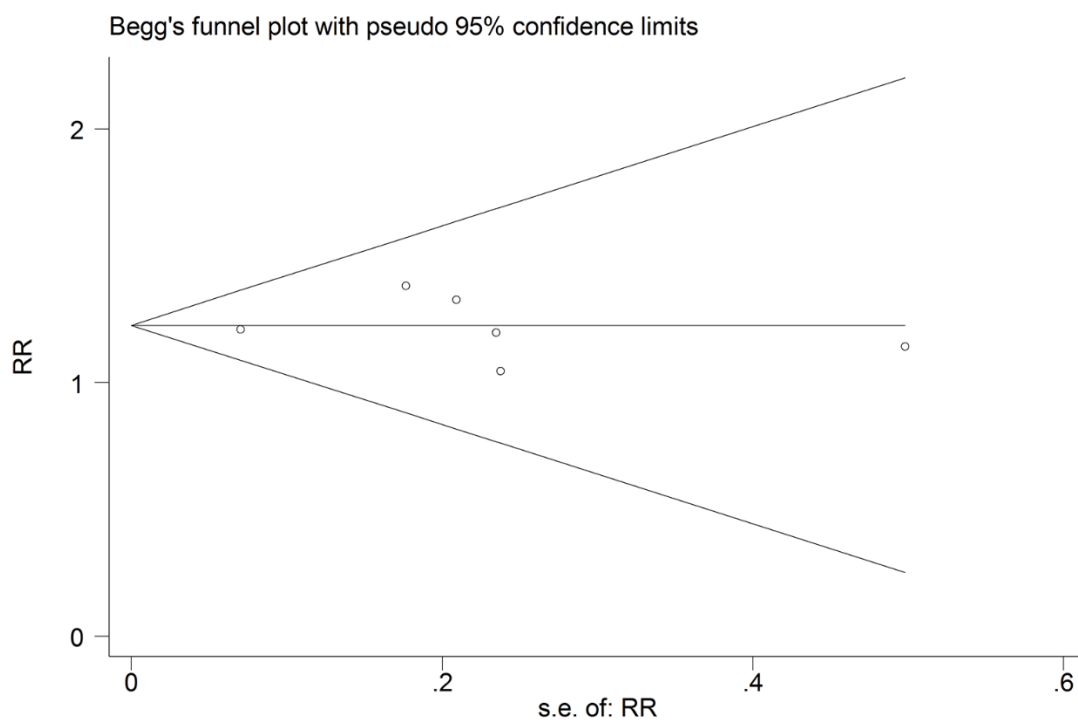
Figure S2. Begg's funnel plot for TP53 rs1042522 polymorphism in malignant bone tumors.
