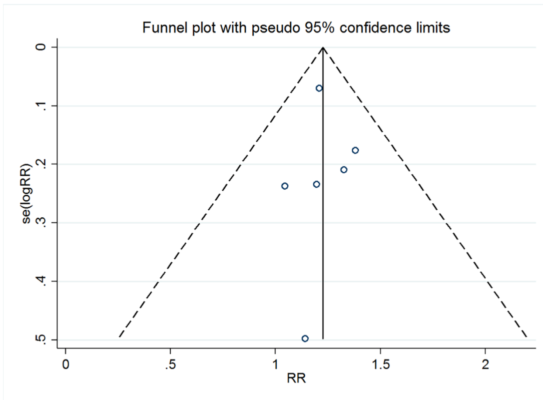
Figure S1. Funnel plot for TP53 rs1042522 polymorphism in malignant bone tumors.
