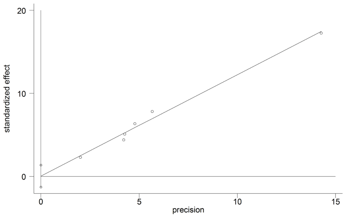
Egger's publication bias plot
